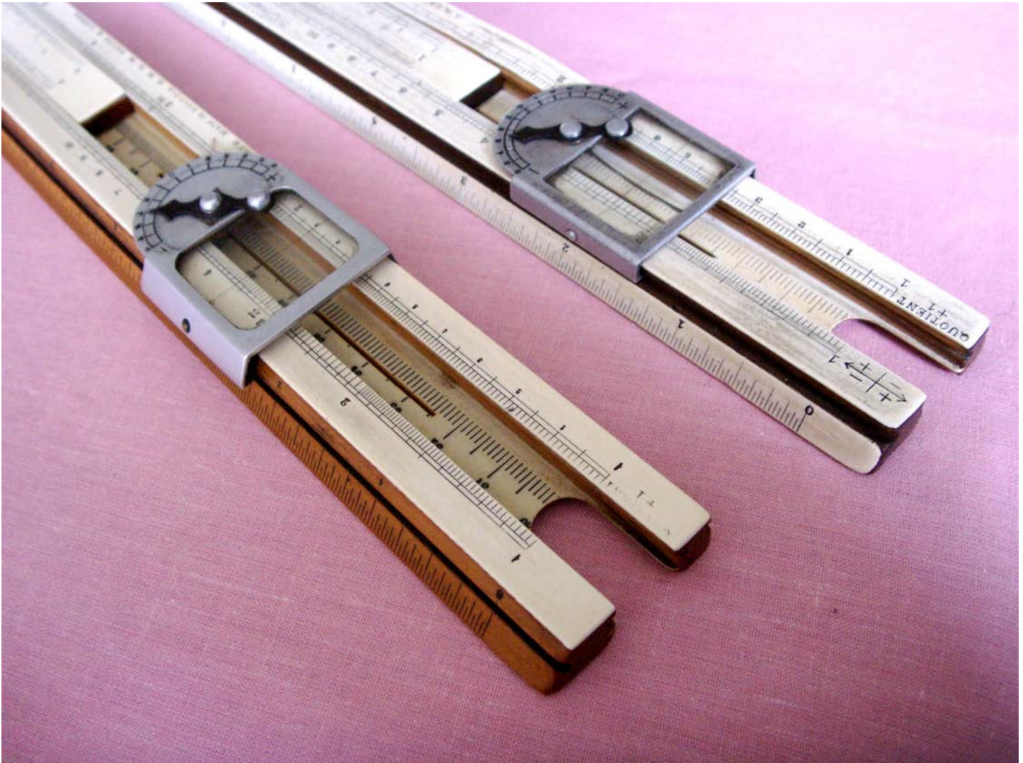
Figure 3. Old (left) and new (right) styles of digit-registering cursor and the altered grooves in the inch scale. Note the rounded (old) and squared (new) corners to the cursor glass. Note also the plastic on the new inch scale, different fonts for the digits, slits in the well, indents at the end of the well, and the aids to placing the decimal point on the end of the new rule (similar marks on the old rule have been almost rubbed away.)
